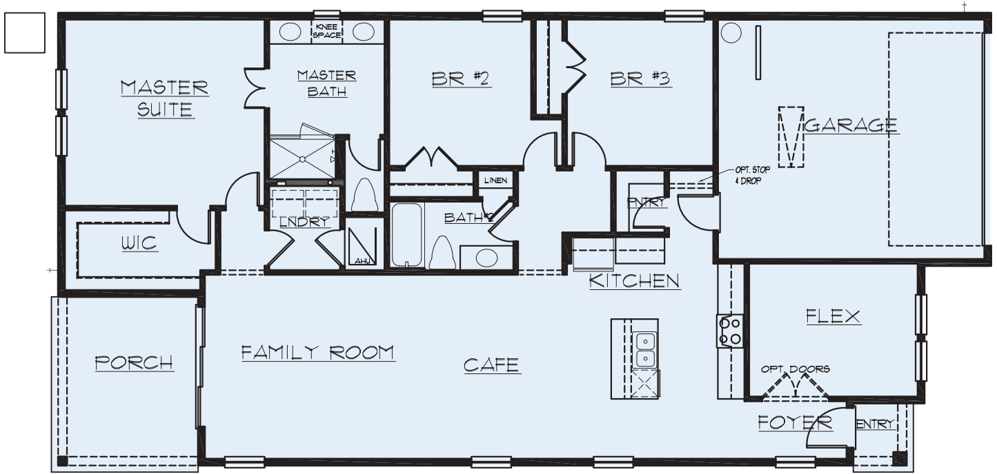
FLOOR PLAN - A
