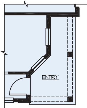
FLOOR PLAN - B
