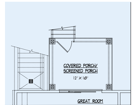
Optional Covered Porch off Great Room
